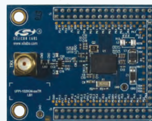
Si1020 UNIVERSAL DEVELOPMENT PLATFORM DAUGHTER CARD
